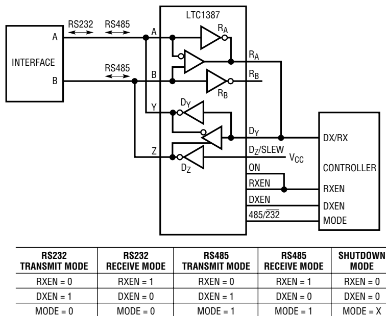
Figure 13. Half-Duplex RS232 (1-Channel), Half-Duplex RS485
