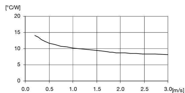
Thermal resistance vs. airspeed measured at the converter. Tested in wind tunnel with airflow and test conditions as per the Thermal consideration section.
