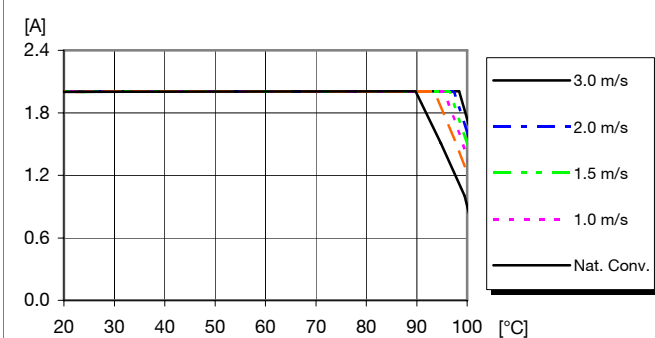
Available load current vs. ambient air temperature and airflow at V_i = 27\text{ V} . See Thermal Consideration section.
