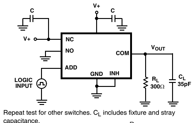
FIGURE 1D. ADDRESS TEST CIRCUIT
