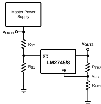
Figure 22. Sequencing Circuit
