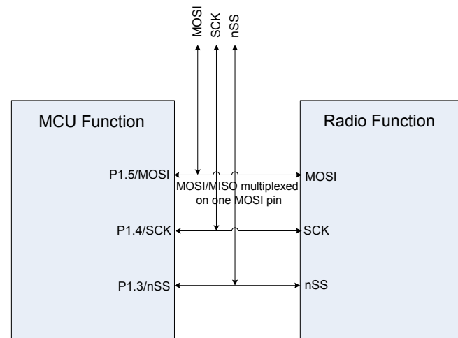
Figure 6. 3-Wire SPI Mode
