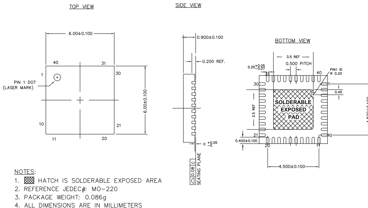
Figure 25. 40-pin QFN (6 × 6 × 1.0 mm) LT40B 3.50 × 3.50 E-Pad (Sawn) Package Outline, 001-13190
