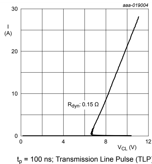
Fig. 5. Dynamic resistance
