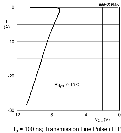
Fig. 6. Dynamic resistance
