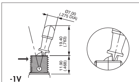
1 locked position (function 6) Typical angle of throw : 26°
