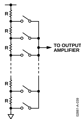
Figure 40. Resistor String
