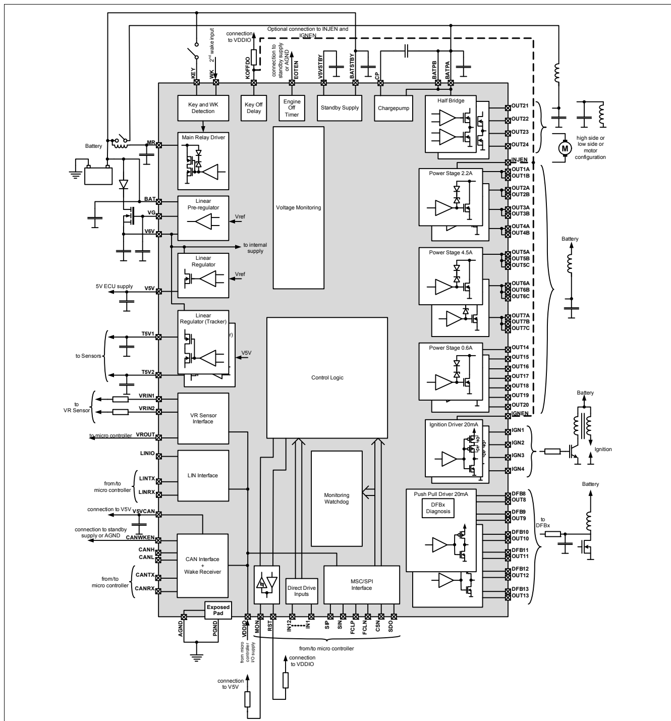
Figure 68 Application Diagram
