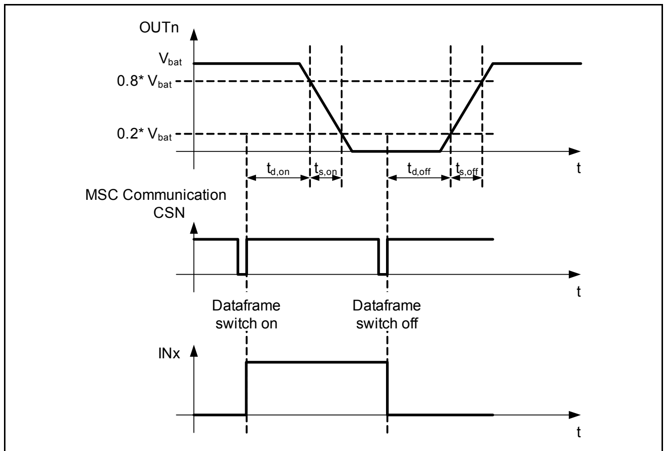
Figure 31 Switching Behavior
