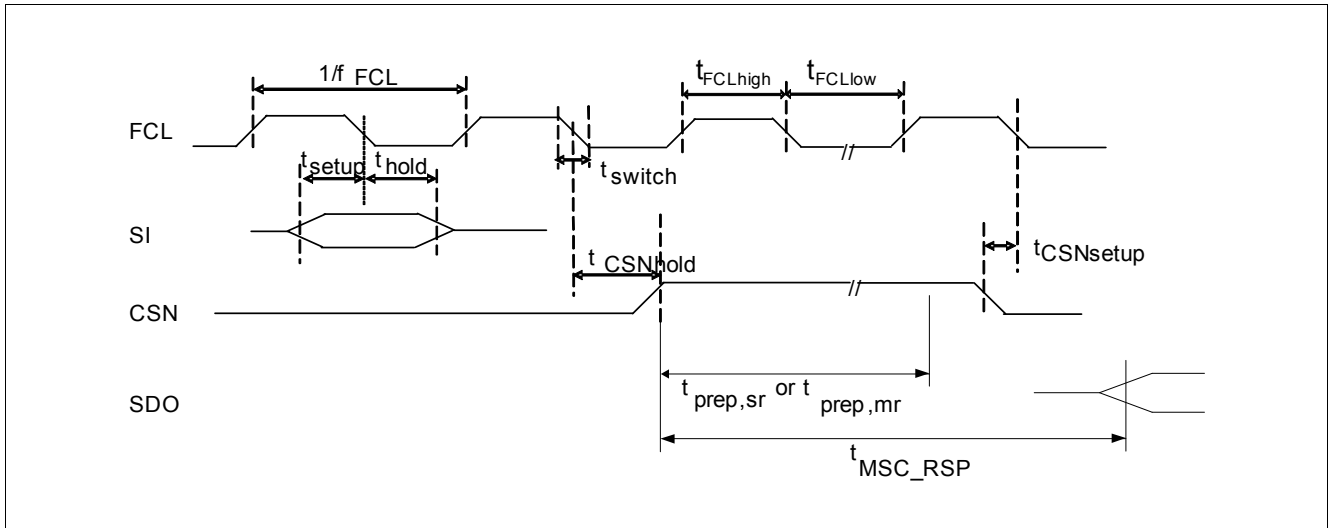
Figure 63 MSC timing
