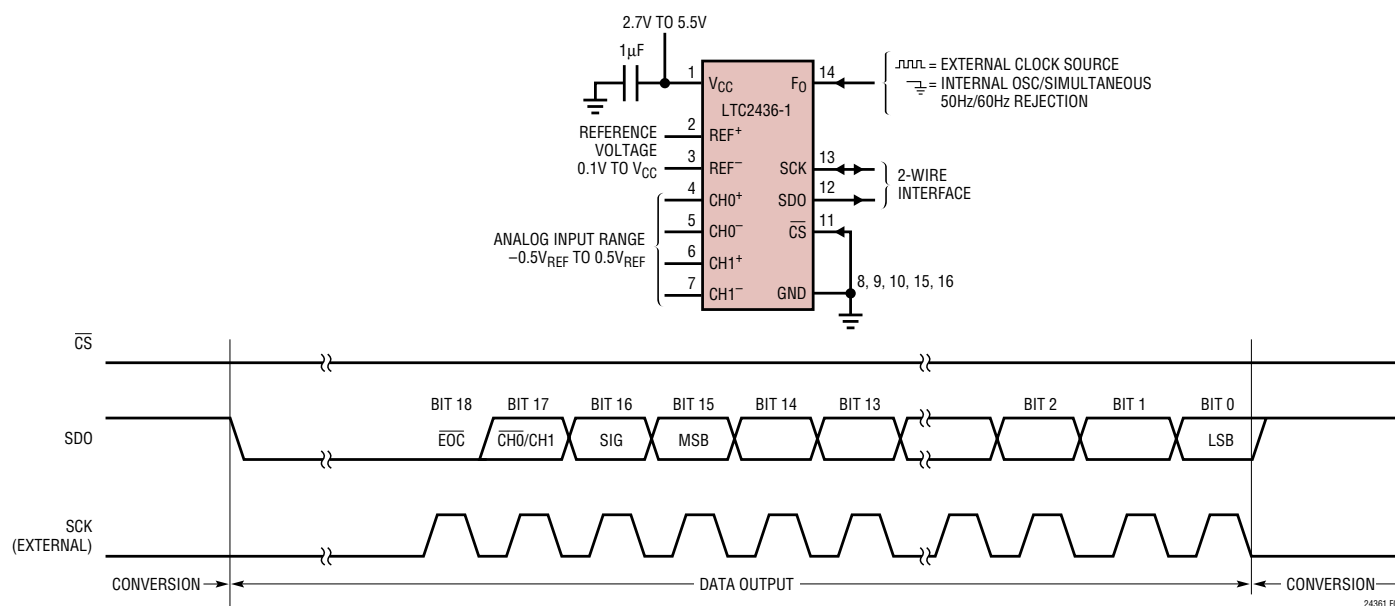
Figure 8. External Serial Clock, \overline{\text{CS}} = 0 Operation (2-Wire)
