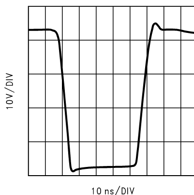
Figure 10. Red Cathode Response
