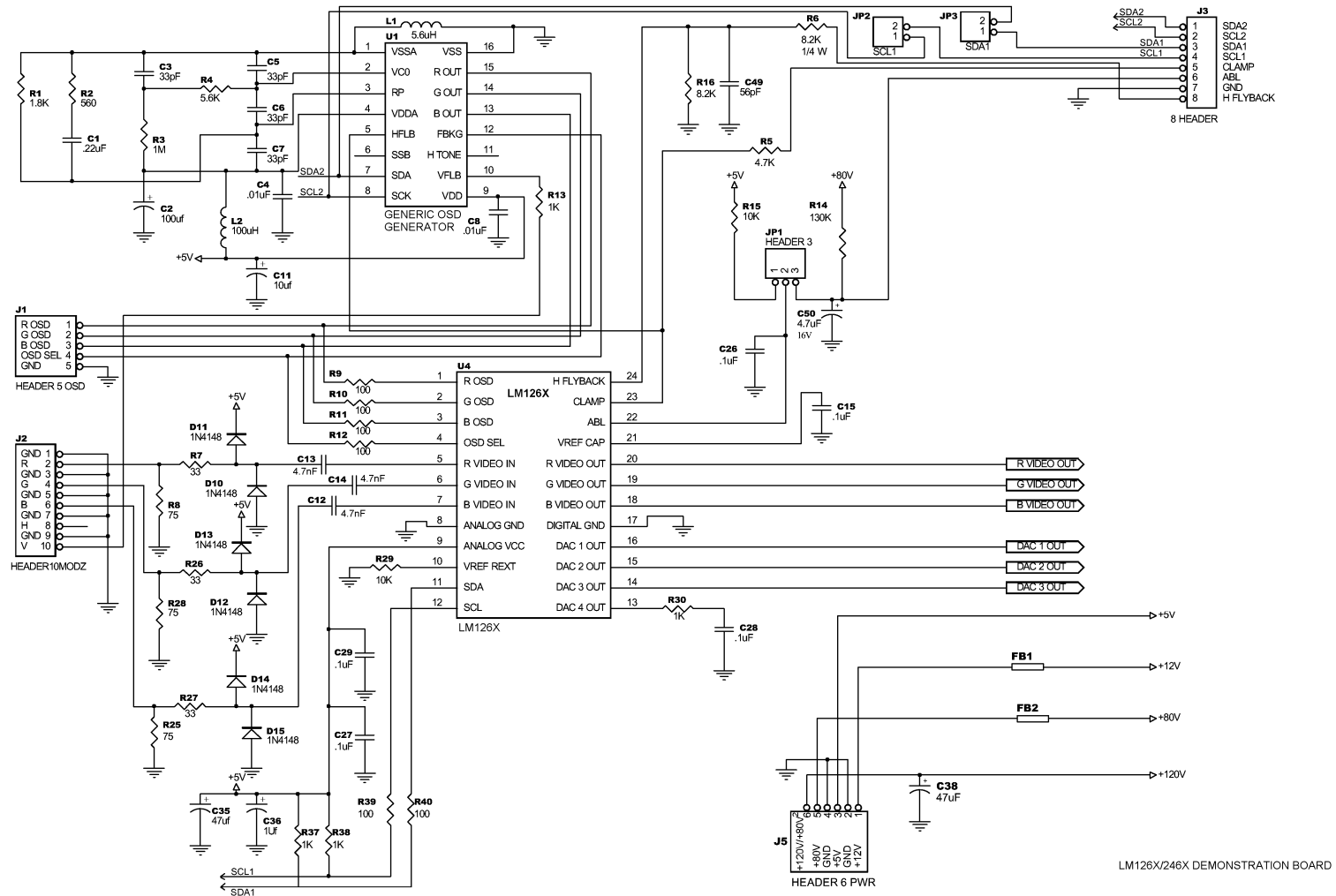
Figure 11. LM126X/LM246X Demonstration Board Schematic
