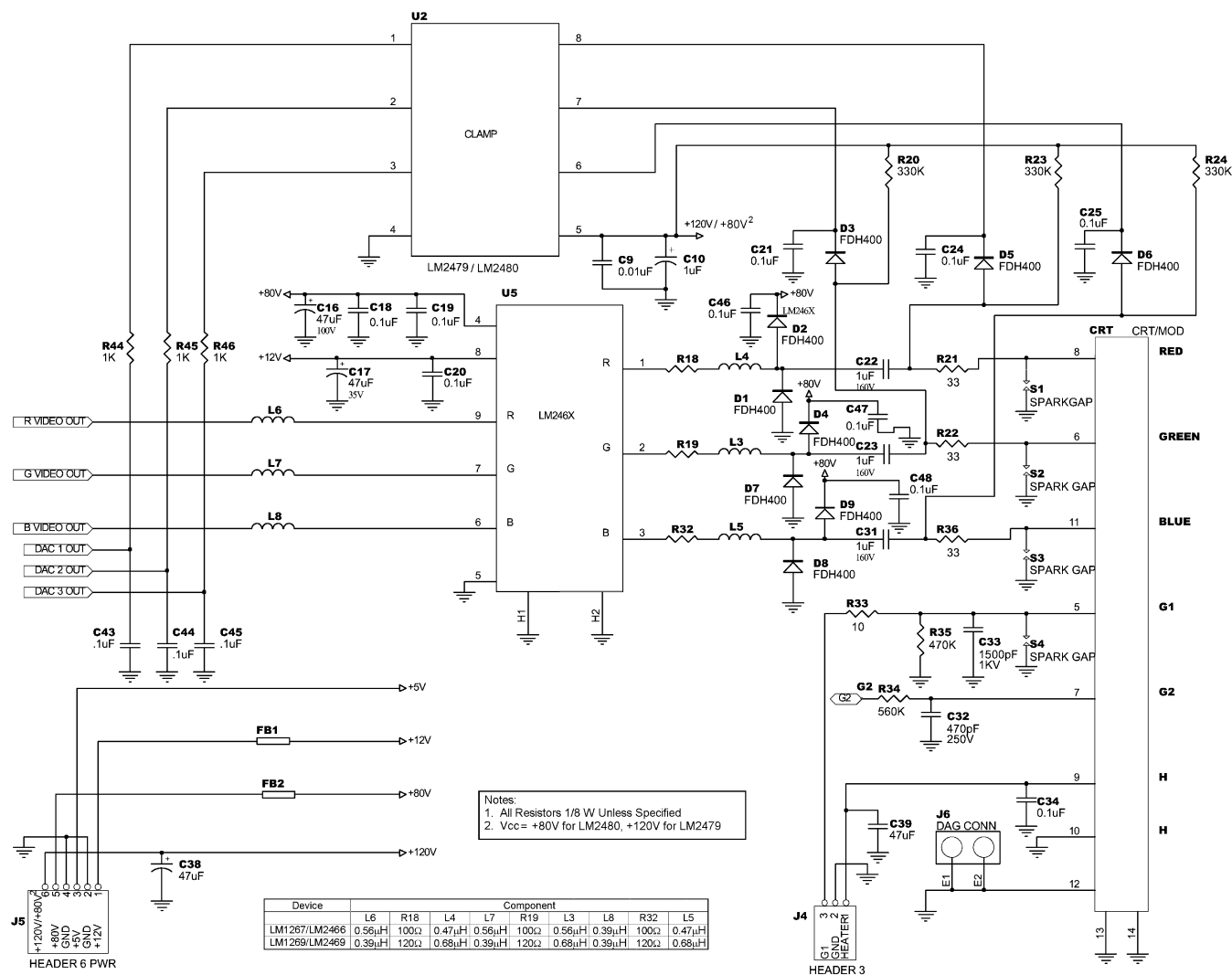
Figure 12. LM126X/LM246X Demonstration Board Schematic (continued)
