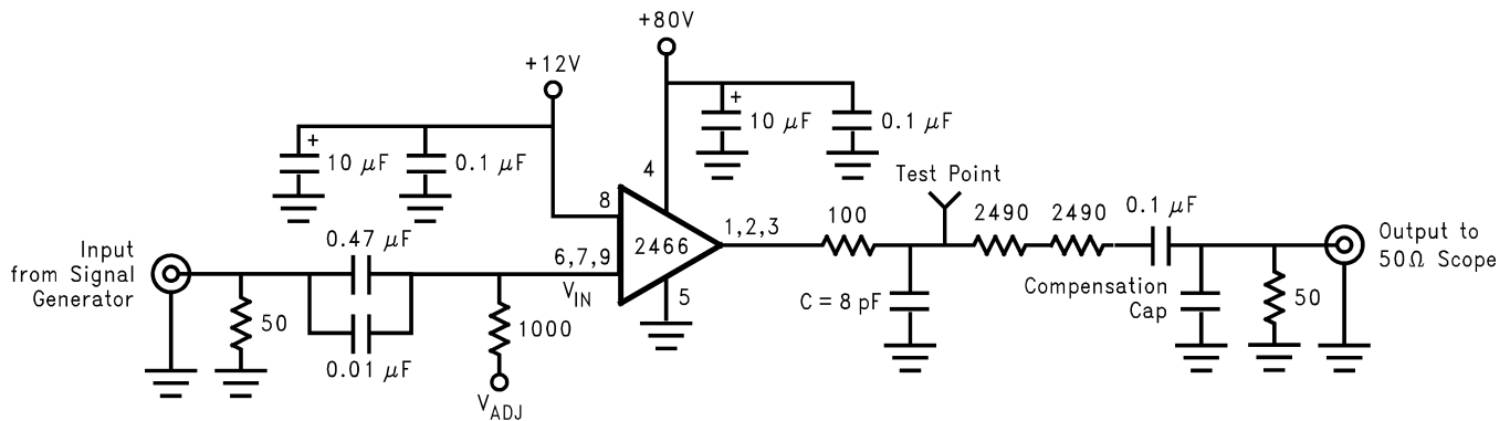
Figure 2. Test Circuit (One Channel)
