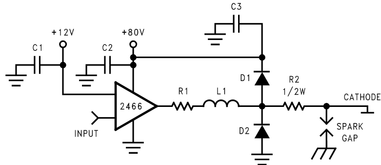
Figure 9. One Channel of the LM2466 with the Recommended Application Circuit
