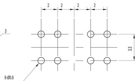
PIERCING PLAN
