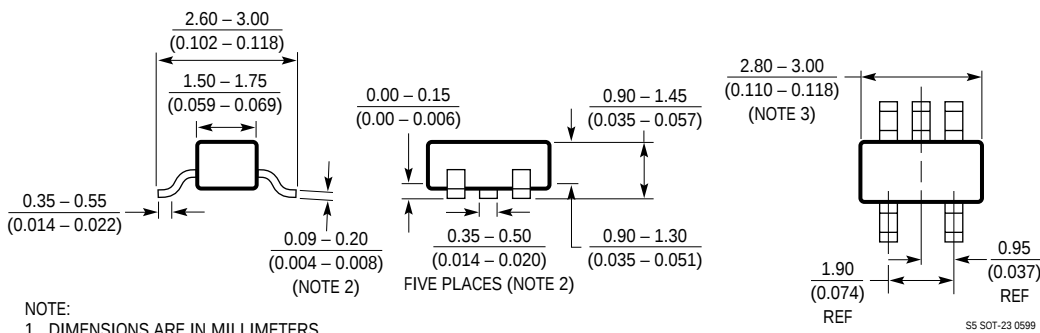
S5 Package 5-Lead Plastic SOT-23 (LTC DWG # 05-08-1633)
