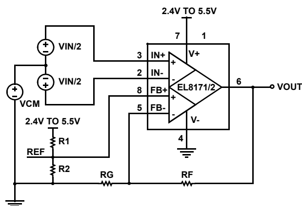
FIGURE 38. CIRCUIT 2 - GAIN SETTING AND REFERENCE CONNECTION
