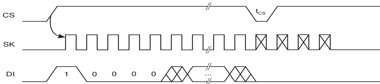
Figure 5. EWDS Timing 1
