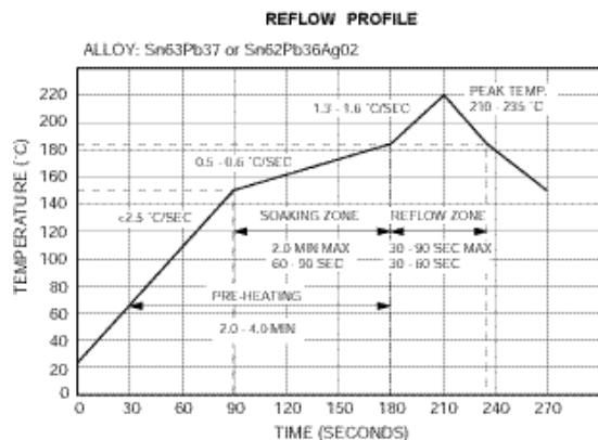
Figure 36. Reflow Profile.
