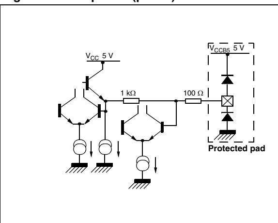
Figure 15. Trap filter (pin 34)
