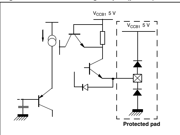
Figure 11. Fast blanking output (pin 49)
