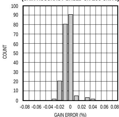
MAX4198 HISTOGRAM (GAIN ACCURACY BASED ON 200 UNITS)
