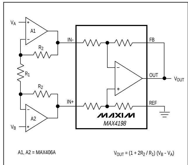
Figure 7. Ultra-Low Input Bias Current (0.1pA) Instrumentation Amplifiers with 47\mu A Supply-Current Consumption
