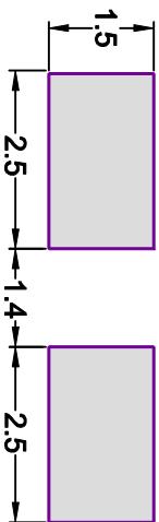
RECOMMENDED DIMENSIONS FOR PC-BOARD PAD
