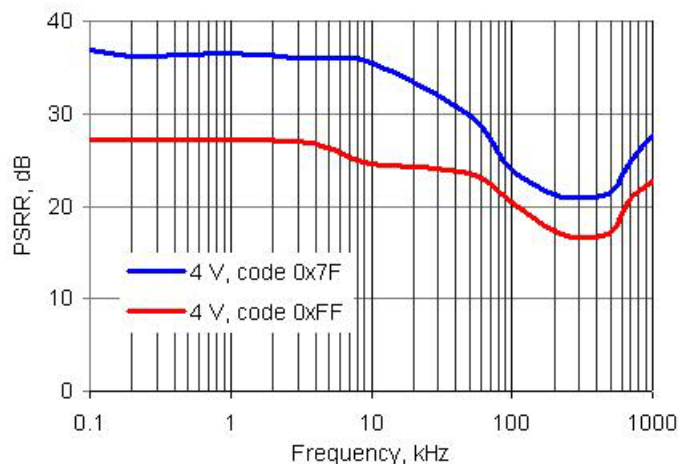
Figure 11-53. VDAC PSRR vs Frequency
