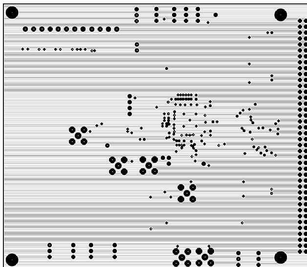
Figure 20. PCB Ground Layer
