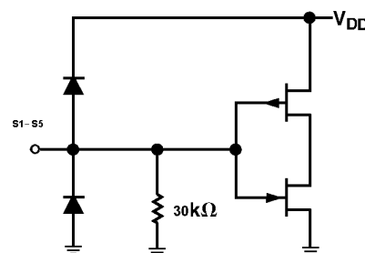
Figure X S1-S5 Inputs
