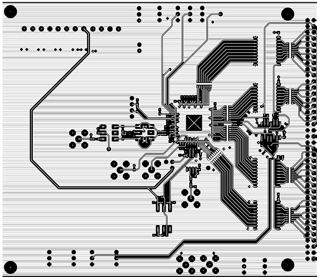
Figure 19. PCB Top Side Copper
