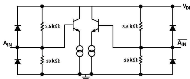
Figure X Analog Inputs
