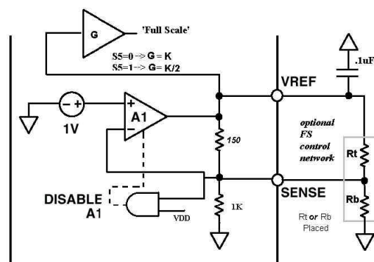
Figure X VREF, SENSE I/O
