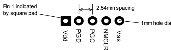
Recommended plate-through connector design
