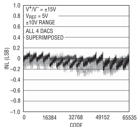
LTC2704-16 Integral Nonlinearity (INL)
