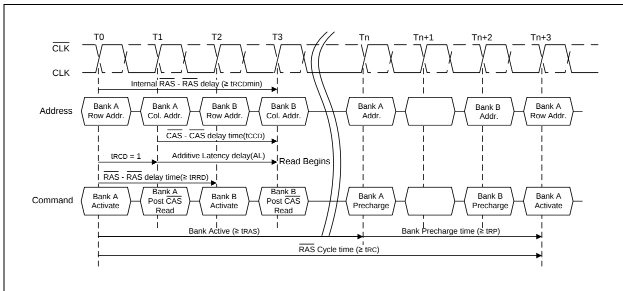
Figure 12 – Bank activate command cycle: \text{trCD} = 3 , \text{AL} = 2 , \text{trP} = 3 , \text{trRD} = 2 , \text{tCCD} = 2
