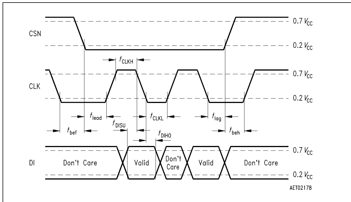
Figure 13 SPI-Input Timing
