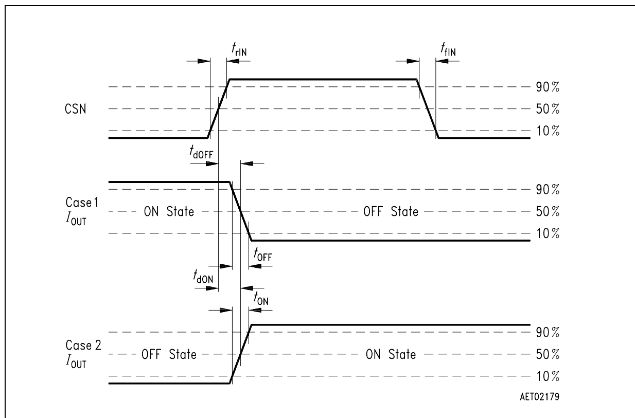
Figure 14 Turn OFF/ON Time
