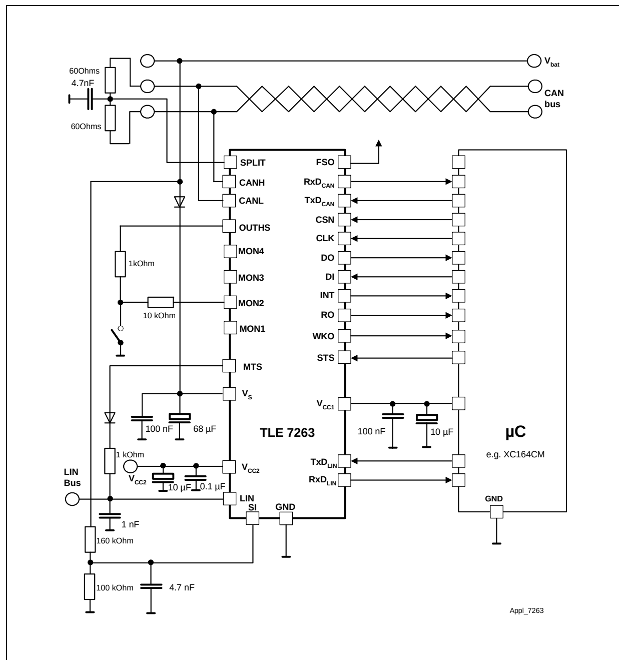
Figure 22 Application Circuit
