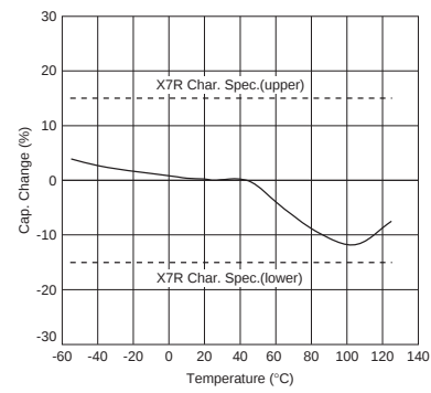
X7R Characteristics
