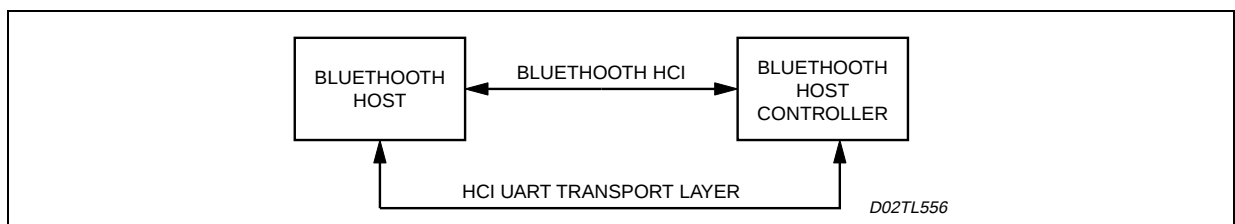
Figure 9. UART Transport Layer
