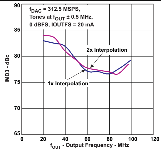
Figure 10. IMD3 vs Interpolation
