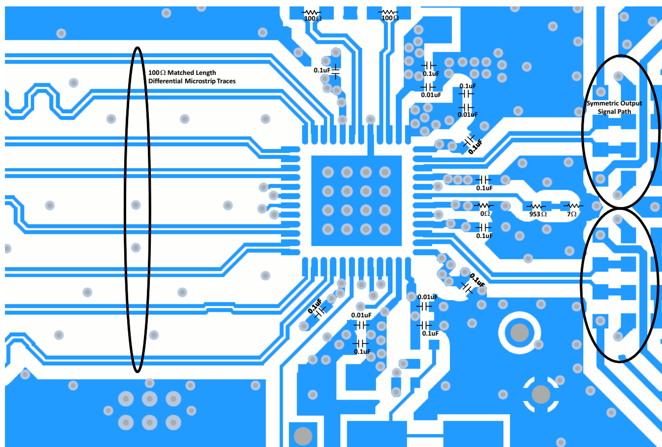
Figure 93. Layout Example
