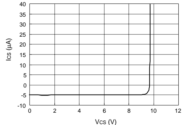
I CS pin current (I CS ) vs. I CS pin voltage (V CS ) FB=open
