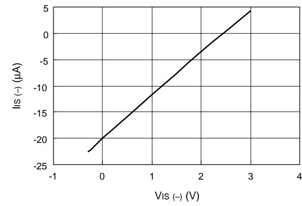
I S (-) pin current (I S (-)) vs. I S (-) pin voltage (V IS (-)) FA5514/15
