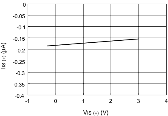
I S (+) pin current (I S (+)) vs. I S (+) pin voltage (V IS (+)) FA5510/11
