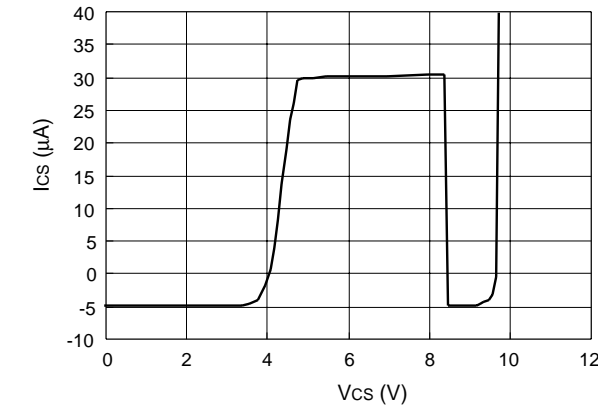
I CS pin current (I CS ) vs. I CS pin voltage (V CS ) FB=0V
