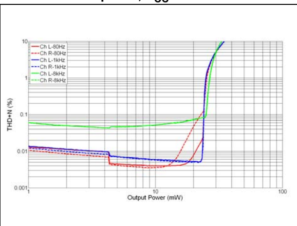
Figure 31. THD+N vs. output power - R_L = 47 \Omega , in-phase, V_{CC} = 3.6 V
