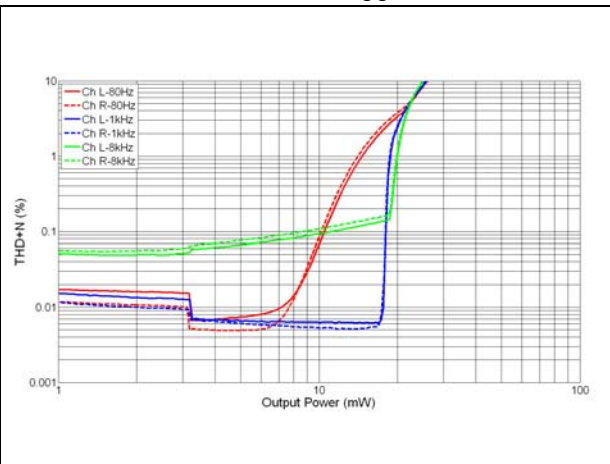
Figure 27. THD+N vs. output power - R_L = 32 \Omega +IPad, in-phase, V_{CC} = 4.8 V
