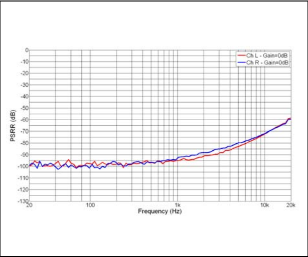
Figure 53. PSRR vs. frequency - V_{CC} = 3.6\text{ V} , gain = 0 dB
