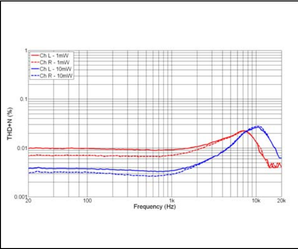
Figure 52. THD+N vs. frequency, R_L = 47\ \Omega , out-of-phase, V_{CC} = 4.8\text{ V}
