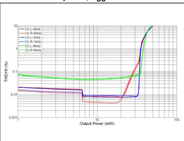
Figure 21. THD+N vs. output power - R_L = 32 \Omega , in-phase, V_{CC} = 4.8 \text{ V}
