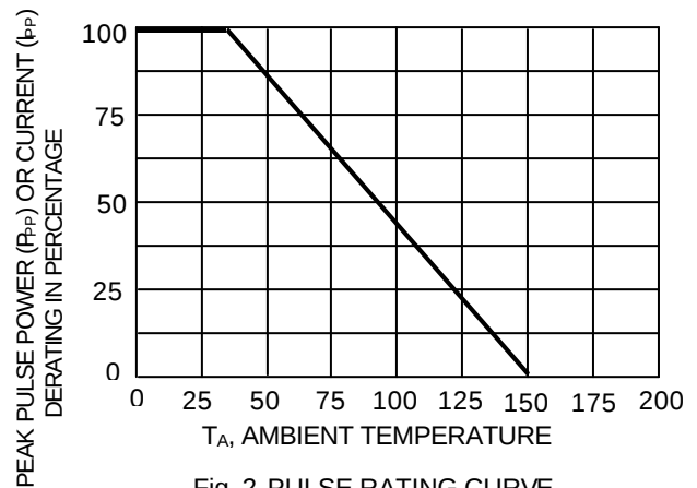
Fig. 2-PULSE RATING CURVE
