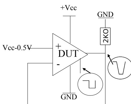
Figure 17. Test configuration for turn-off time (Vout pulled down)
