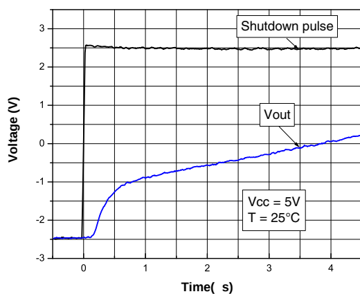
Figure 18. Turn-on time, V_{CC} = 5 V, Vout pulled down, T = 25^\circ\text{C}
