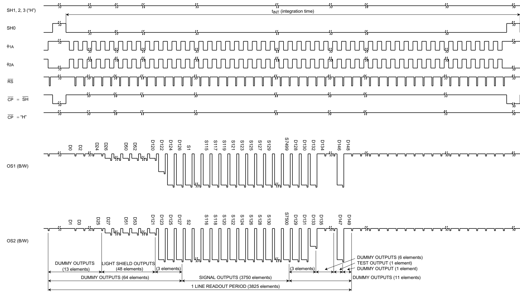
Timing Chart 4: Line Clamp Mode (B/W mode)
