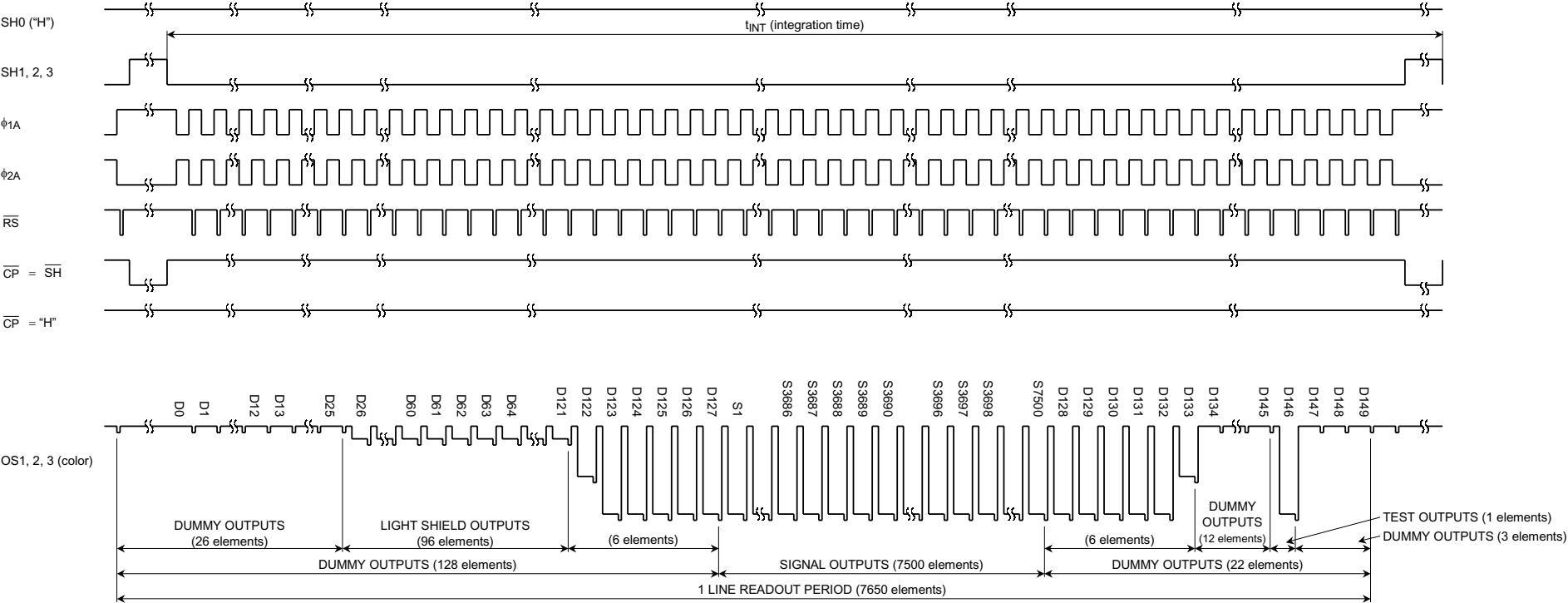
Timing Chart 2: Line Clamp Mode (Color mode)
