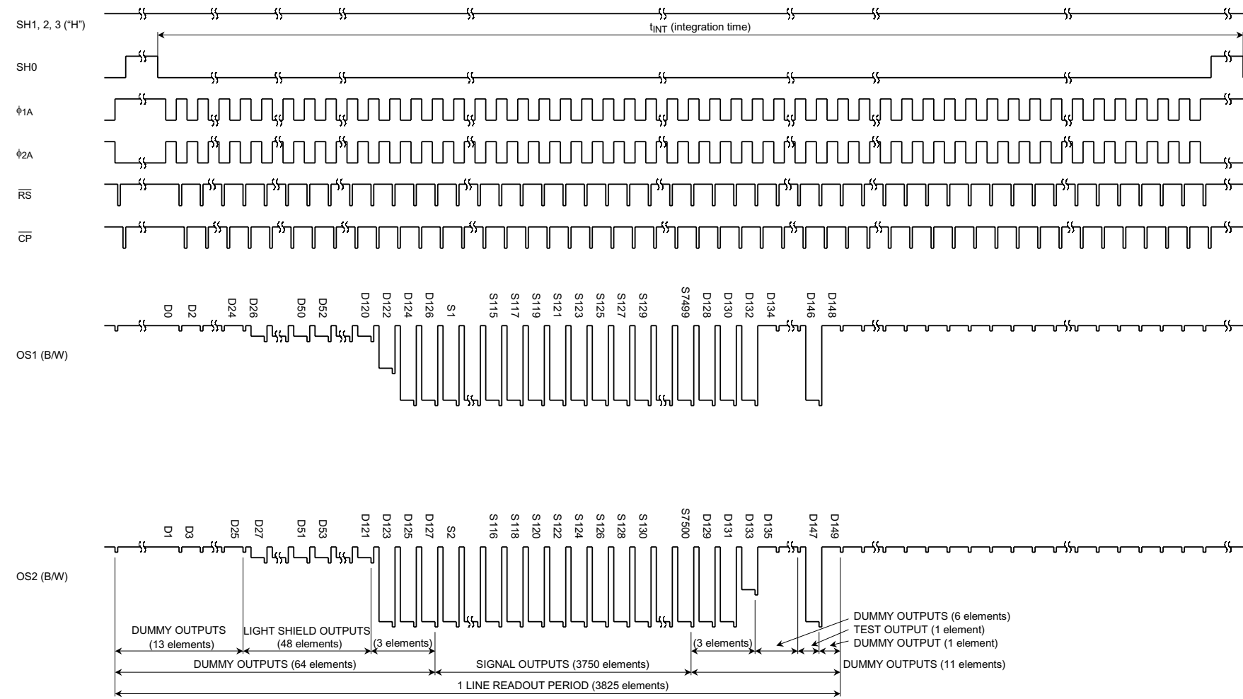
Timing Chart 3: Bit Clamp Mode (B/W mode)
