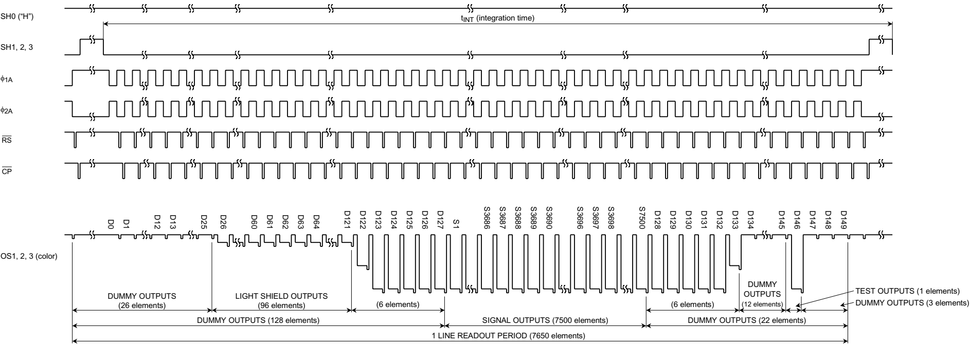
Timing Chart 1: Bit Clamp Mode (Color mode)
