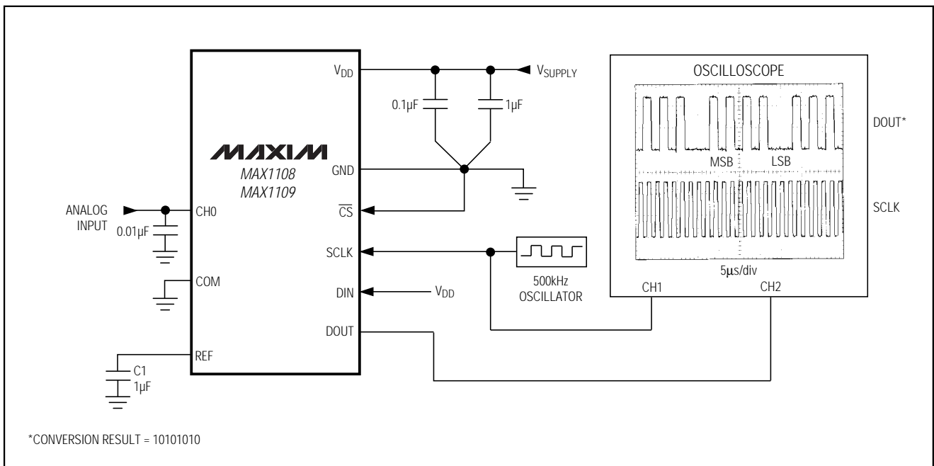
Figure 9. Quick-Look Schematic
