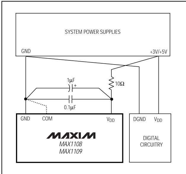
Figure 13. Power-Supply Connections
