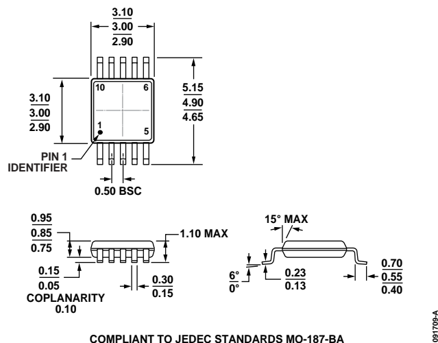
Figure 67. 10-Lead Mini Small Outline Package [MSOP] (RM-10)
