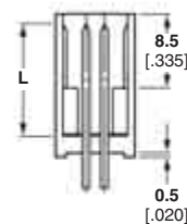
Section X-X
