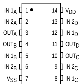
MC14011B Quad 2-Input NAND Gate
