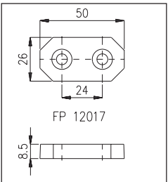
FP 12017 fastening lug measures
