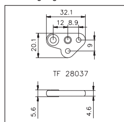
TF 28037 fastening lug measures
