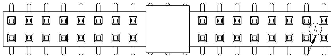
10065490-XXXAXXLF TOP VIEW SEE NOTE 7
