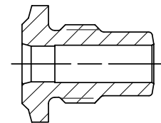
126302 DRIVING ANVIL -08
