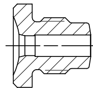
126299 DRIVING ANVIL -06
