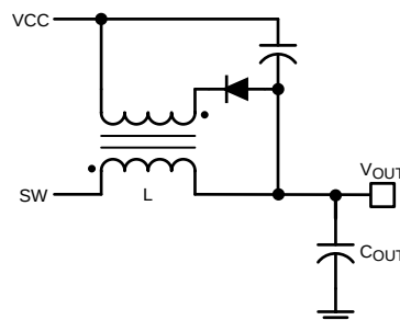
Figure 8. VCC Bias Supply With Additional Inductor Winding
