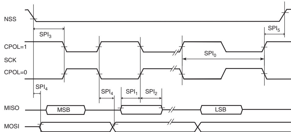
Figure 35-16. USART SPI Master Mode
