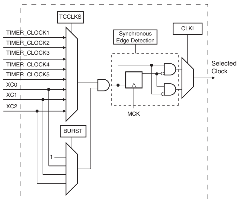
Figure 31-3. Clock Selection
