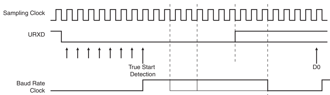
Figure 29-4. Character Reception
