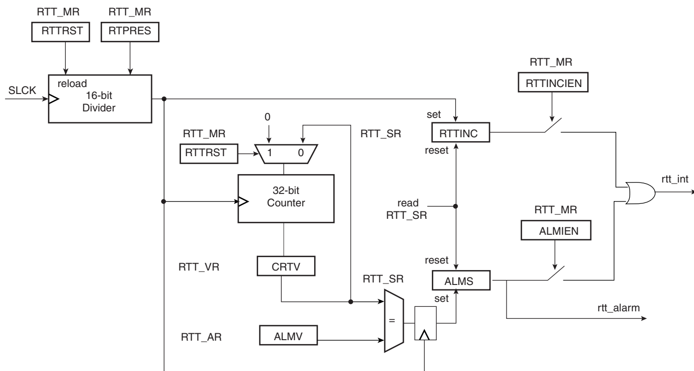
Figure 13-1. Real-time Timer
