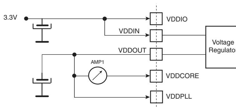
Figure 35-8. Active Mode Measurement Setup
