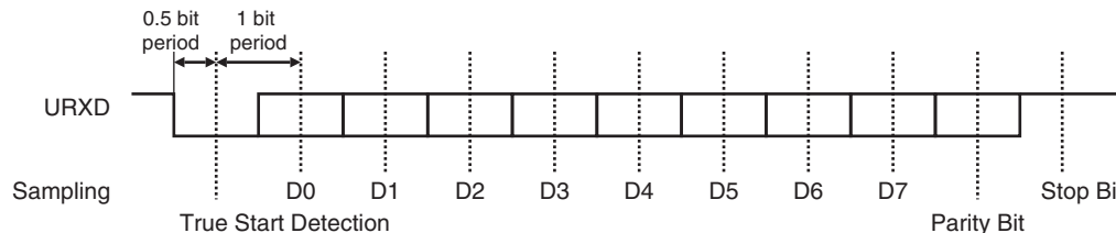
Figure 29-4. Character Reception
