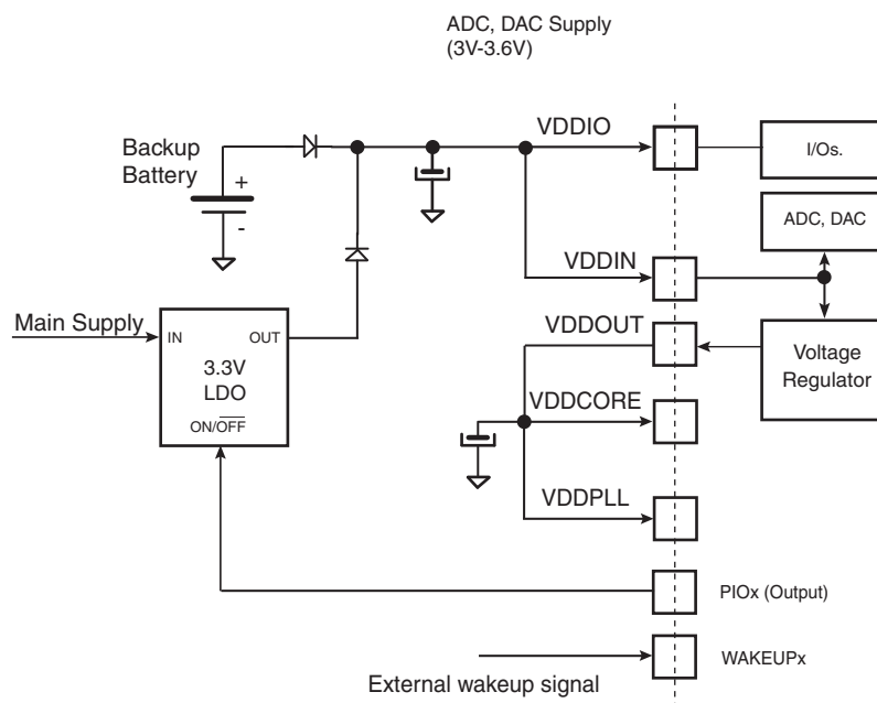
Figure 5-3. Core Externally Supplied (backup battery)
