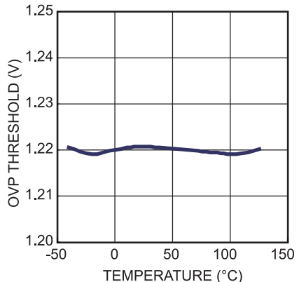
OVP Threshold vs. T_J
