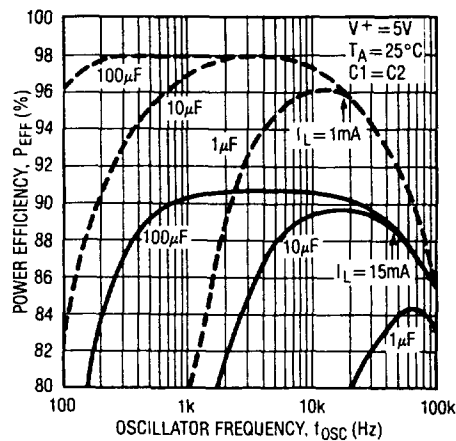
Power Efficiency vs Oscillator Frequency
