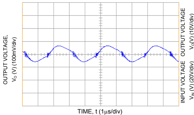
Figure 2. Typical Output Ripple and Noise at Room Temperature and 48Vin; I o = I o,max ; C o,ext = 470μF.
