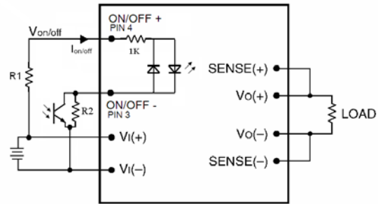
Figure 10. Circuit configuration for using Remote On/Off Implementation.
