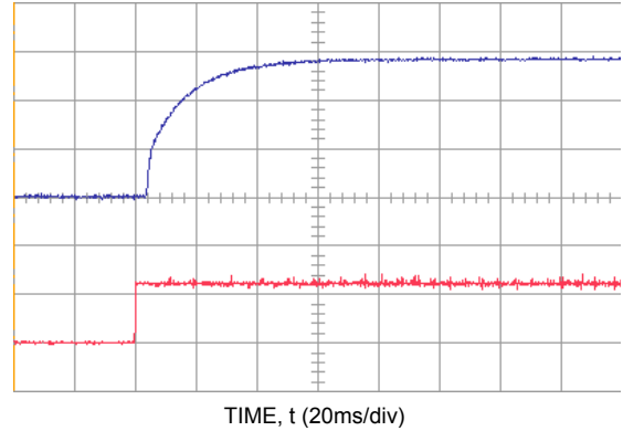
Figure 4. Typical Start-Up Using Remote On/Off, R1=30Kohm; C o,ext = 470μF.
