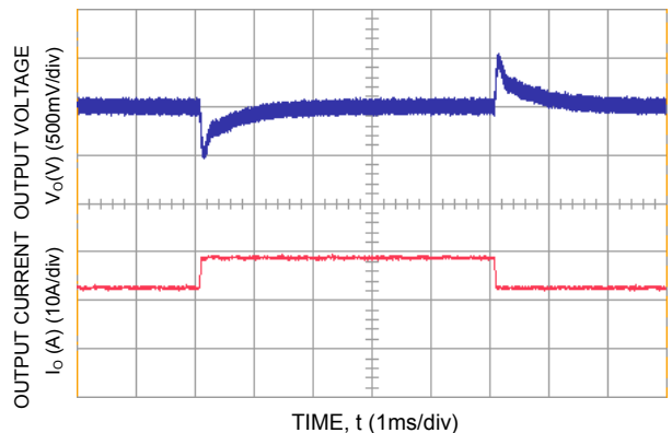
Figure 6. Transient Response to Dynamic Load Change from 50% to 75% to 50% of Full Load at Room Temperature and 48 Vdc Input; 0.1A/μS ; C o,ext = 470μF.
