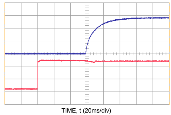
Figure 5. Typical Start-Up Using from V IN , positive logic version shown; C o,ext = 470μF.
