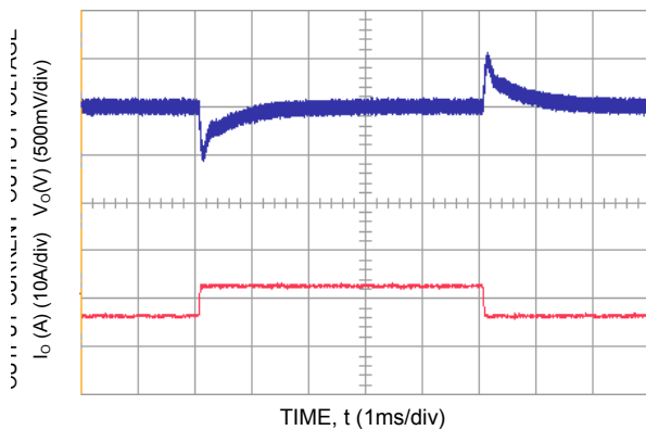
Figure 3. Transient Response to Dynamic Load Change from 25% to 50% to 25% of Full Load at Room Temperature and 48 Vdc Input; 0.1A/μS ; C o,ext = 470μF.
