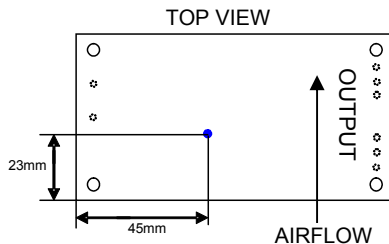
Figure 14. Case ( T_C ) Temperature Measurement Location (top view).
