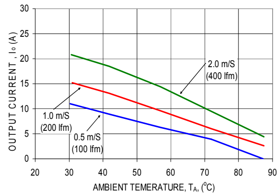
Figure 16. Derating Output Current vs. Local Ambient Temperature and Airflow, No Heatsink, V_{IN} = 48\text{V} .
