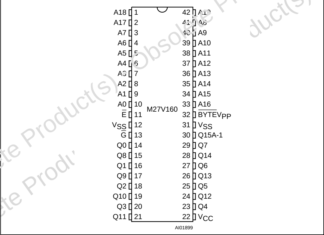
Figure 2. DIP Connections
