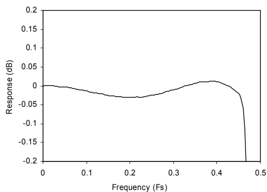
Figure 39 DAC Digital Filter Ripple
