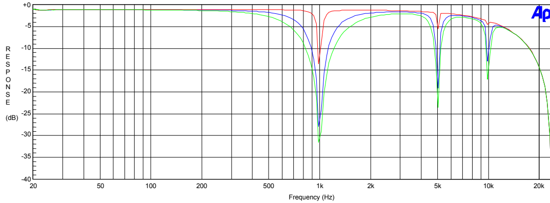
Figure 48 Cumulative Notch + Low Pass Filters Responses (48kHz); NF0 f_c = 1\text{kHz} ; NF1 f_c = 5\text{kHz} ; NF2 f_c = 10\text{kHz} ; LPF f_c = 11\text{kHz} ; f_b = 100\text{Hz} , 600\text{Hz} , 2\text{kHz}
