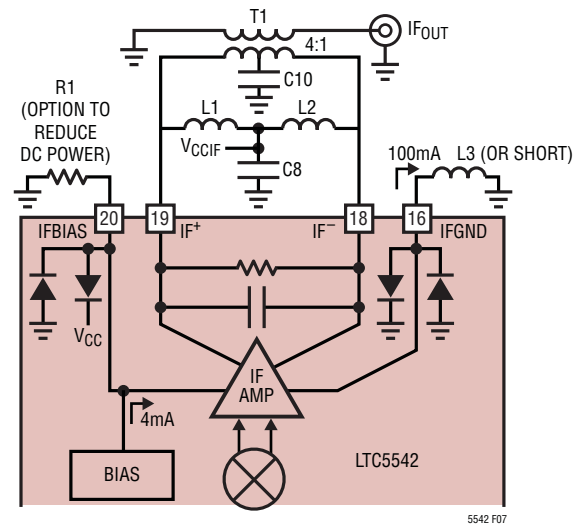
Figure 7. IF Amplifier Schematic with Bandpass Match
