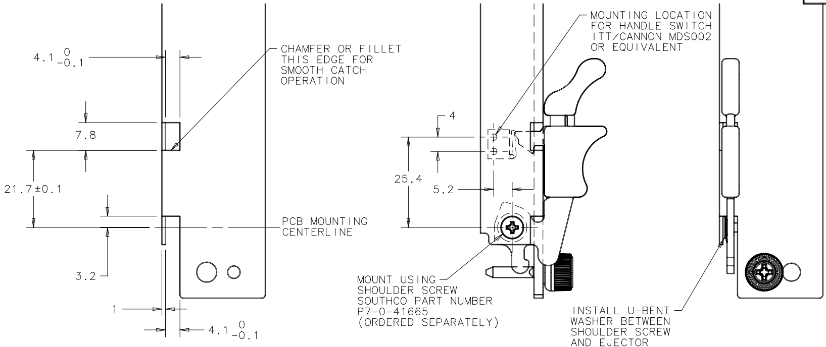
PANEL PREPARATION FACEPLATE THICKNESS 2.5mm
