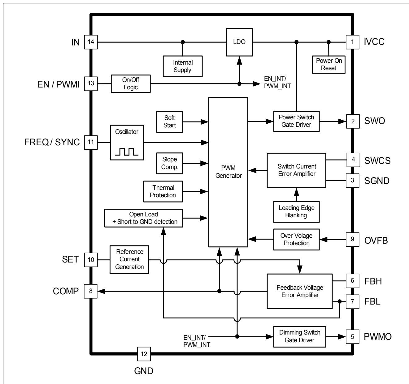
Figure 1 Block Diagram
