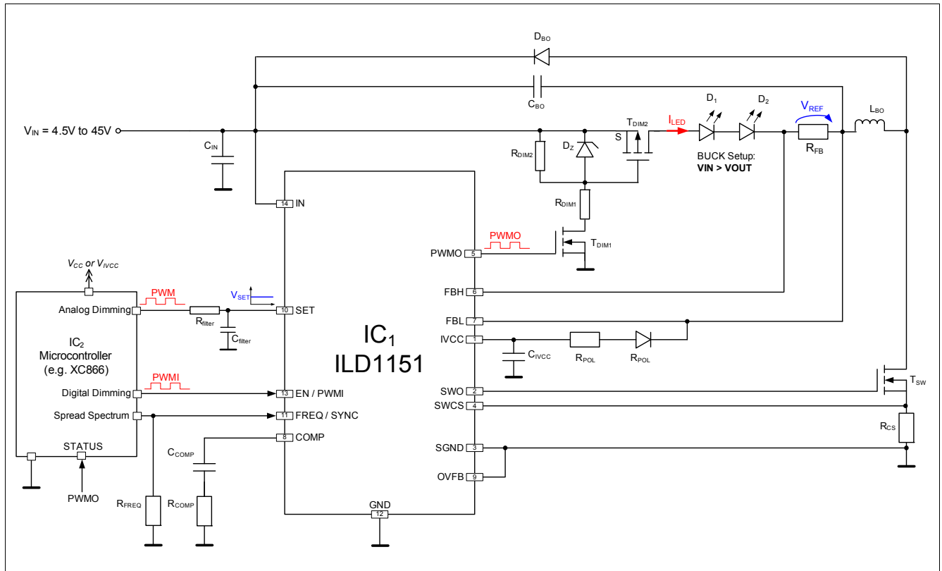
Figure 27 Buck Application Circuit + Short Circuit protection
